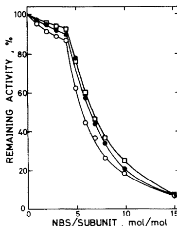
Fig.1. Inactivation of cAsp-AT as a function of NBS to enzyme ratio. ( \square ) Pyridoxal form, ( \circ ) pyridoxamine form, ( \bullet ) apoenzyme. See text for details.
